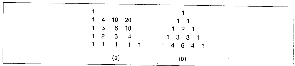
Figure 3.6 Pascal's triangle
